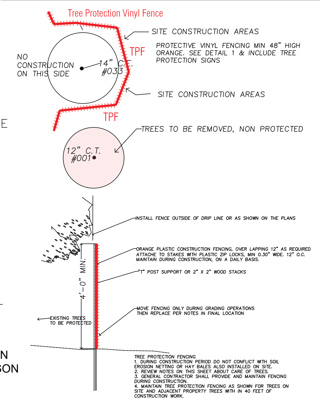
1 TREE PROTECTION FENCE DETAIL NOT TO SCALE
