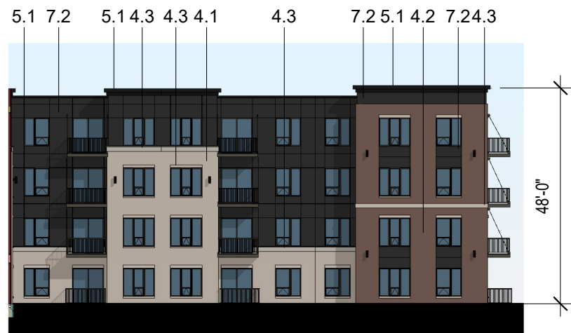
⑤ East Elevation 7 1" = 30'-0"
