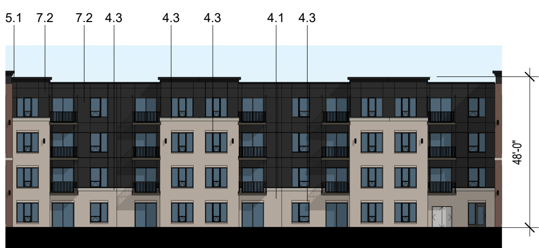
④ West Elevation 4 1" = 30'-0"
