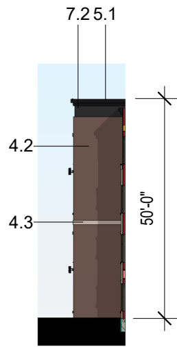
⑤ West Elevation 5 1" = 30'-0"
