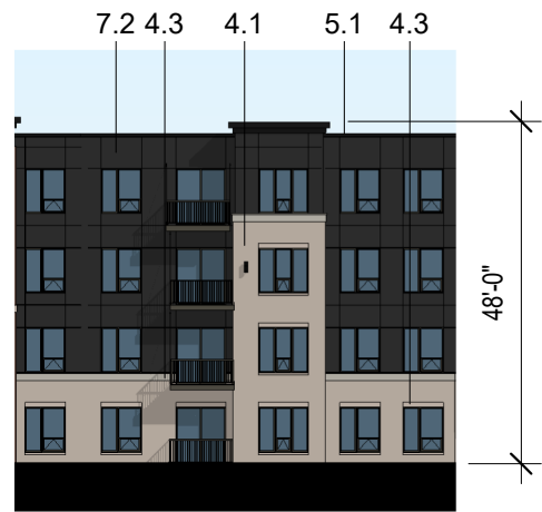
② East Elevation 4 1" = 30'-0"
