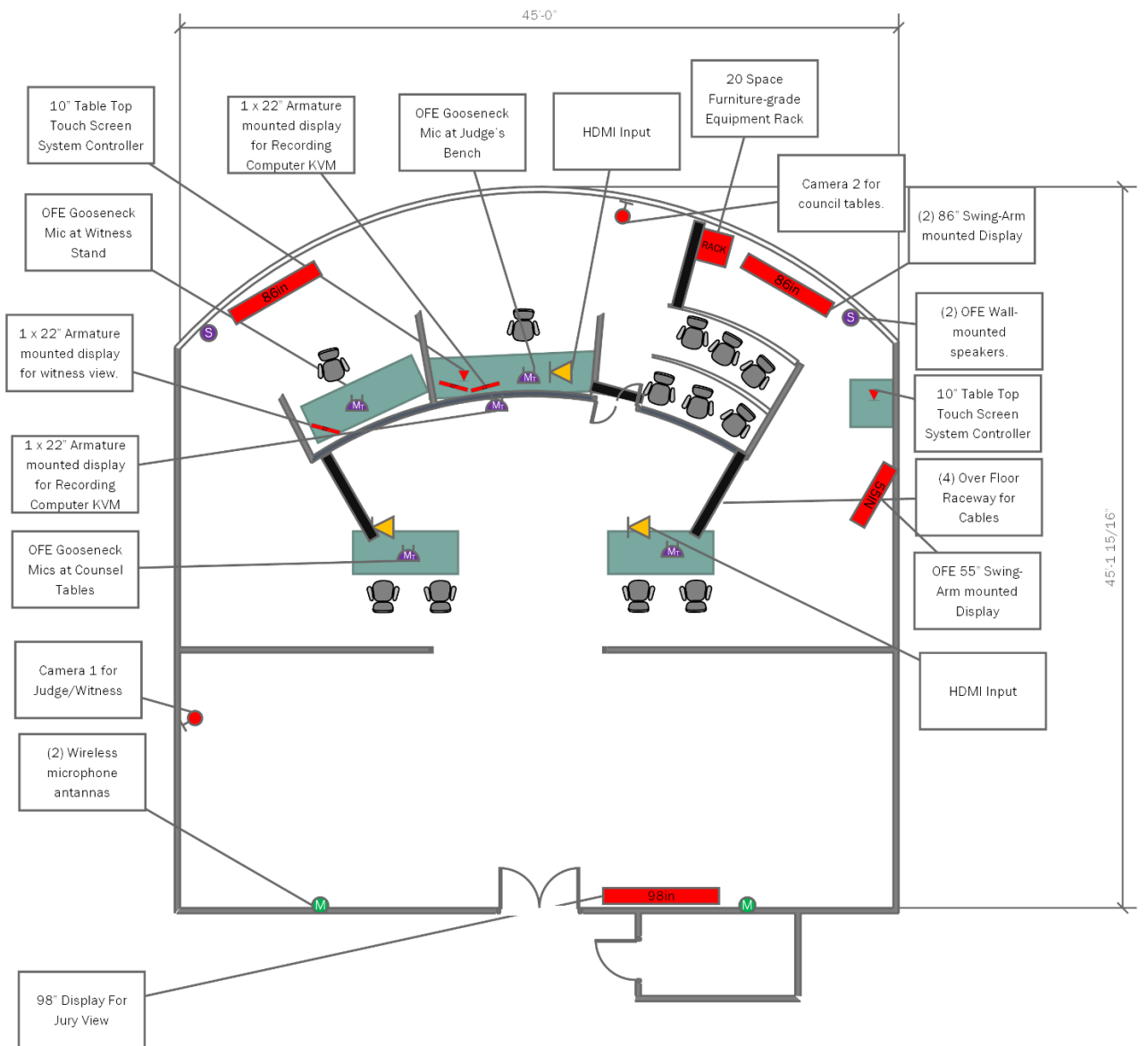
1 Room Layout TAC001 N.T.S. for notation only.
