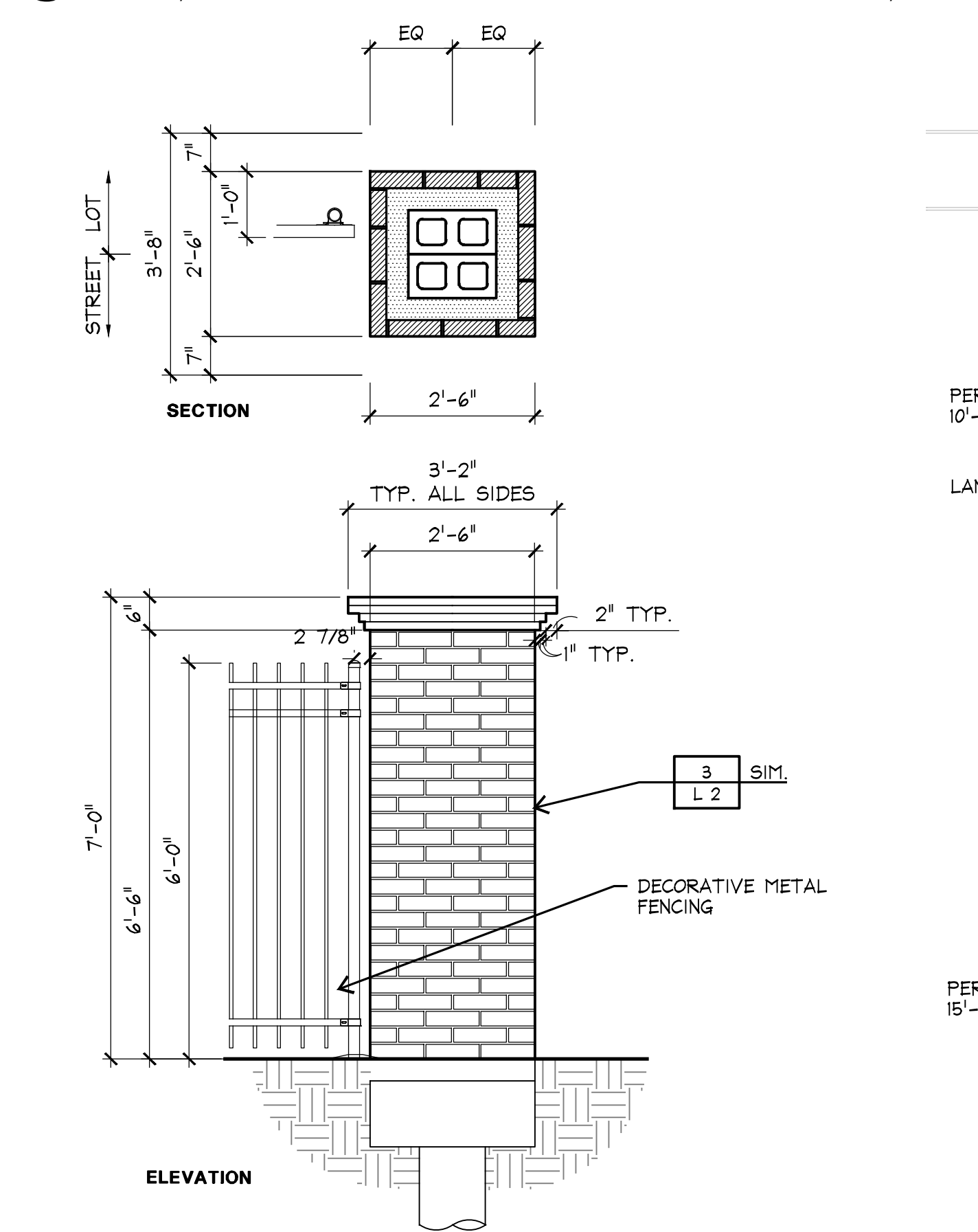
2 FENCE COLUMN AT METAL FENCE SECTION/ELEVATION SCALE: 1/2"=1'-0"
