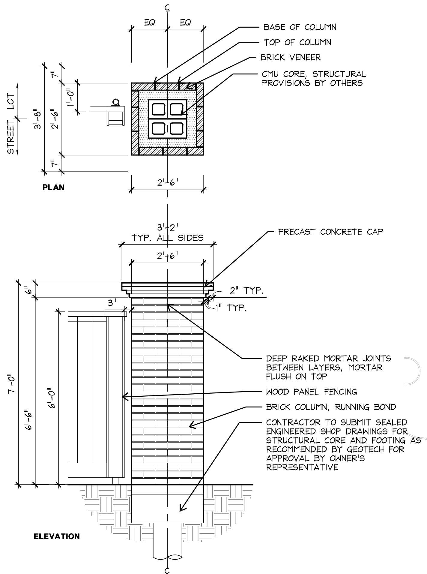
3 FENCE COLUMN AT WOOD FENCE SECTION/ELEVATION SCALE: 1/2"=1'-0"
