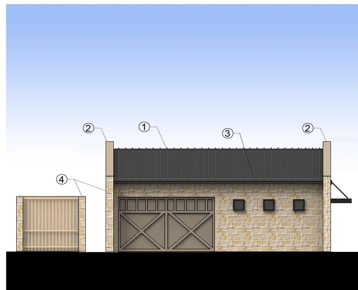
2 SOUTH ELEVATION
