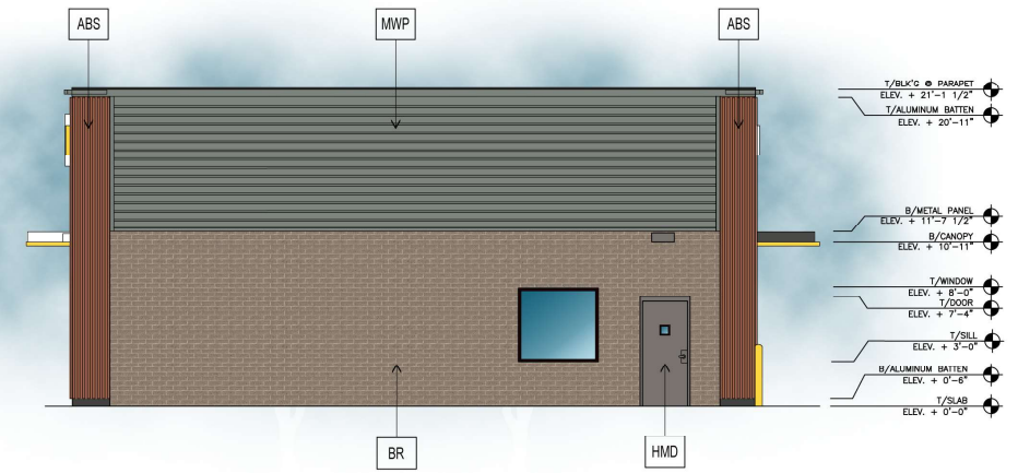
REAR ELEVATION - WEST
