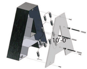
Typical construction isometric
