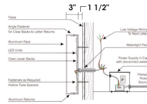
Typical construction details
