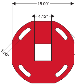
.5" STEEL DRIVE THRU CANOPY BASE PLATE
