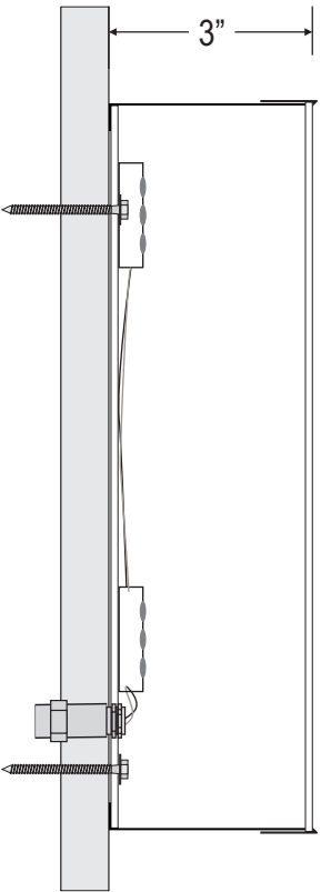
COFFEE & BAKERY SIDE SECTION VIEW SCALE: NTS
