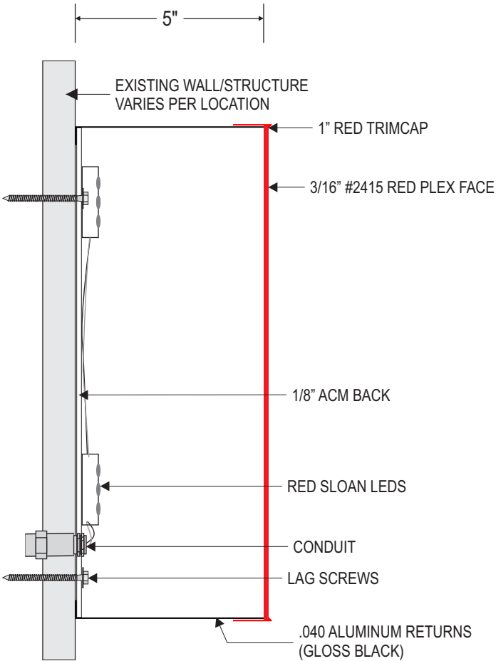
TIM HORTONS SIDE SECTION VIEW SCALE: NTS
