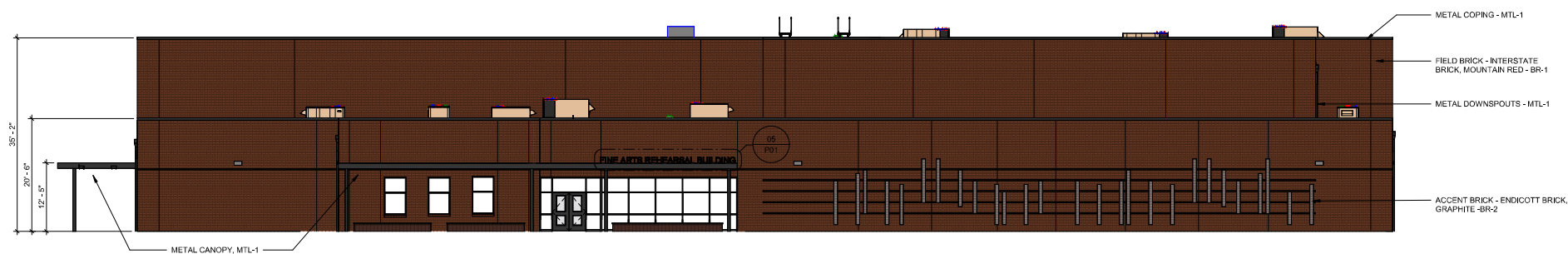
01 EXTERIOR ELEVATION - FINE ARTS OVERALL - NORTH 3/32" = 1'-0"
