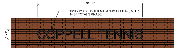
05 ENLARGED ELEVATION - TENNIS BUILDING SIGNAGE 3/8" = 1'-0"
