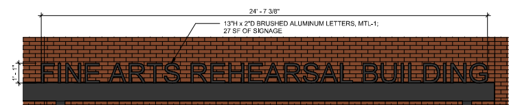
05 ENLARGED ELEVATION - FINE ARTS BUILDING SIGNAGE 3/8" = 1'-0"
