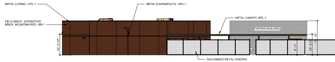
02 EXTERIOR ELEVATION - TENNIS OVERALL - EAST 3/32" = 1'-0"
