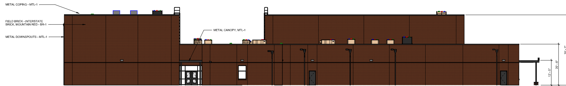
02 EXTERIOR ELEVATION - FINE ARTS OVERALL - EAST 3/32" = 1'-0"
