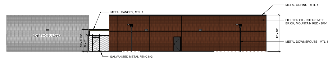
01 EXTERIOR ELEVATION - TENNIS OVERALL - WEST 3/32" = 1'-0"
