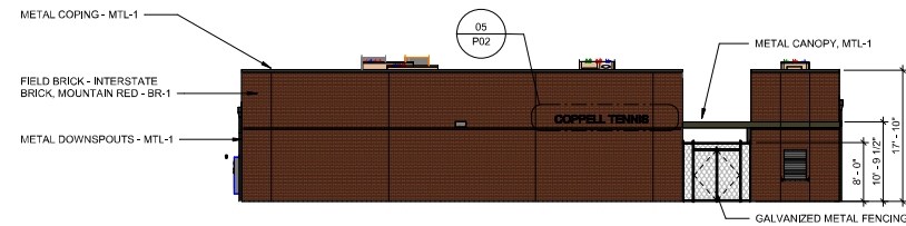
03 EXTERIOR ELEVATION - TENNIS OVERALL - SOUTH 3/32" = 1'-0"
