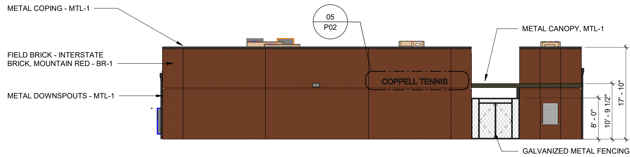
03 EXTERIOR ELEVATION - TENNIS OVERALL - SOUTH 3/32" = 1'-0"
