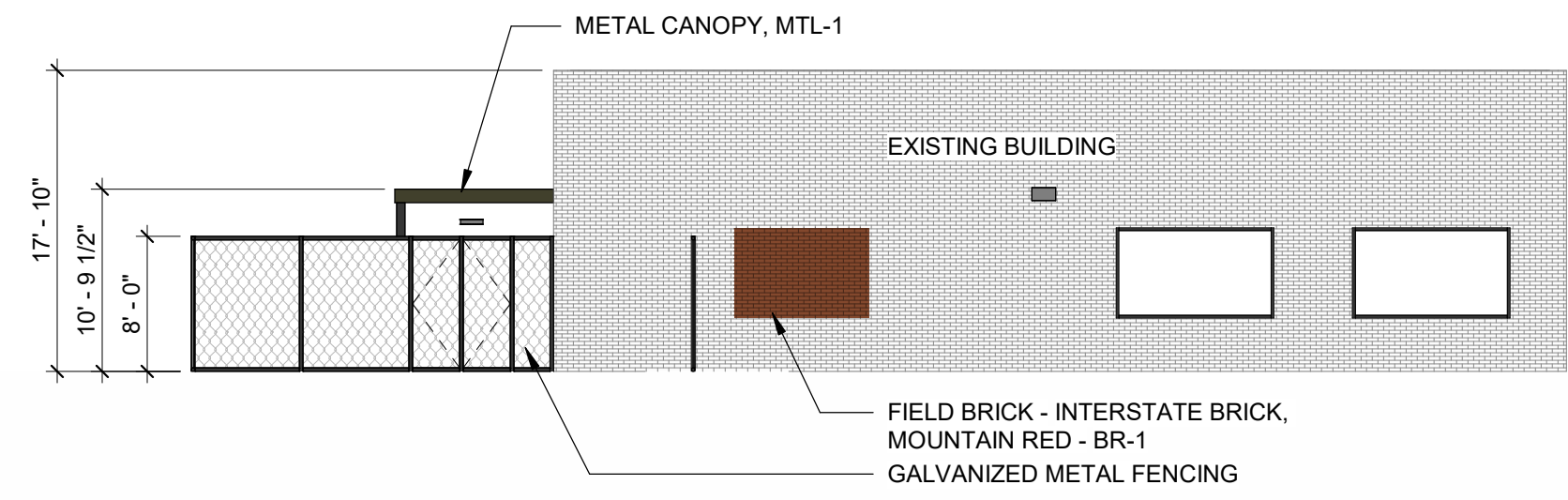
04 EXTERIOR ELEVATION - TENNIS OVERALL - NORTH 3/32" = 1'-0"
