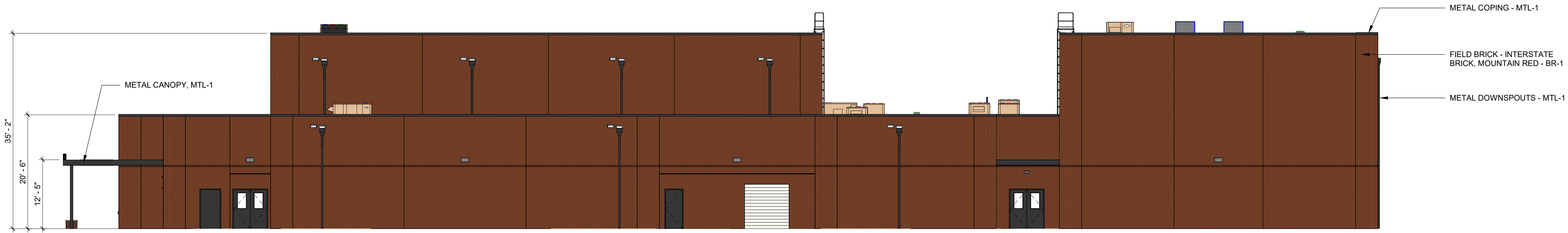
04 EXTERIOR ELEVATION - FINEARTS OVERALL - WEST 3/32" = 1'-0"
