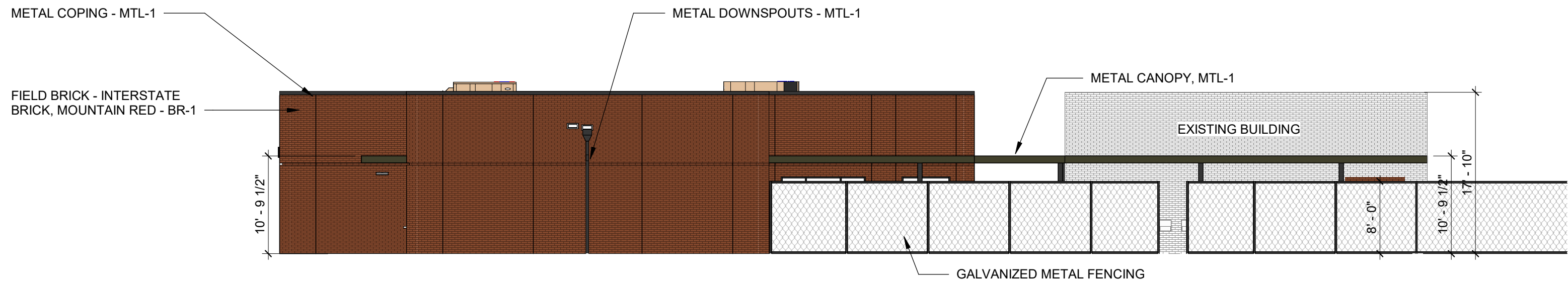
02 EXTERIOR ELEVATION - TENNIS OVERALL - EAST 3/32" = 1'-0"
