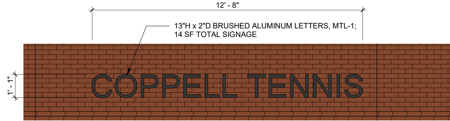
05 ENLARGED ELEVATION - TENNIS BUILDING SIGNAGE 3/8" = 1'-0"
