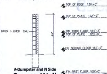
05 A-Dumpster and N Side Screen Wall Section Scale: 3/8" = 1'-0"
