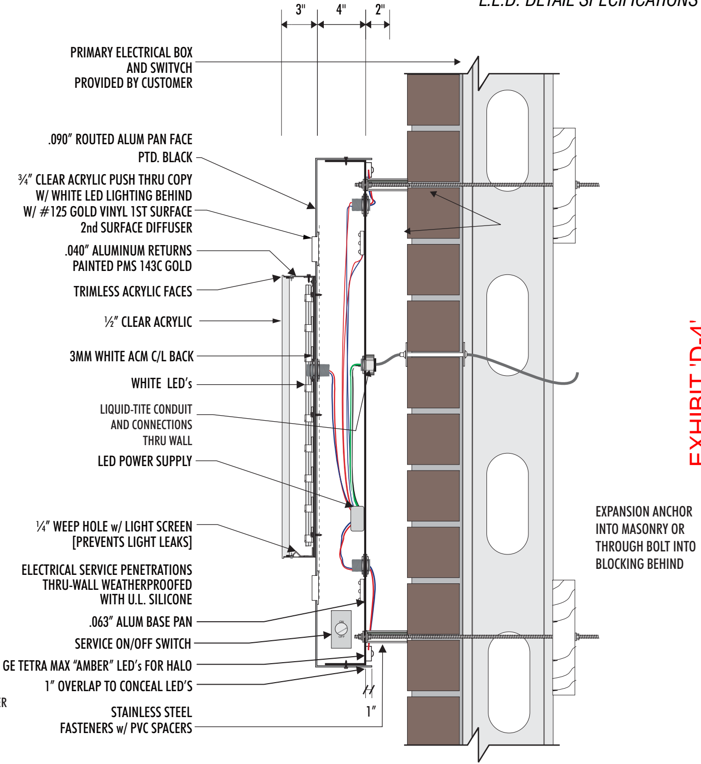
SECTION DRAWING - LED FACE LIT C/L ON FACE LIT & REVERSE HALO LIT CABINET SCALE: 1 1/2" = 1'-0"
