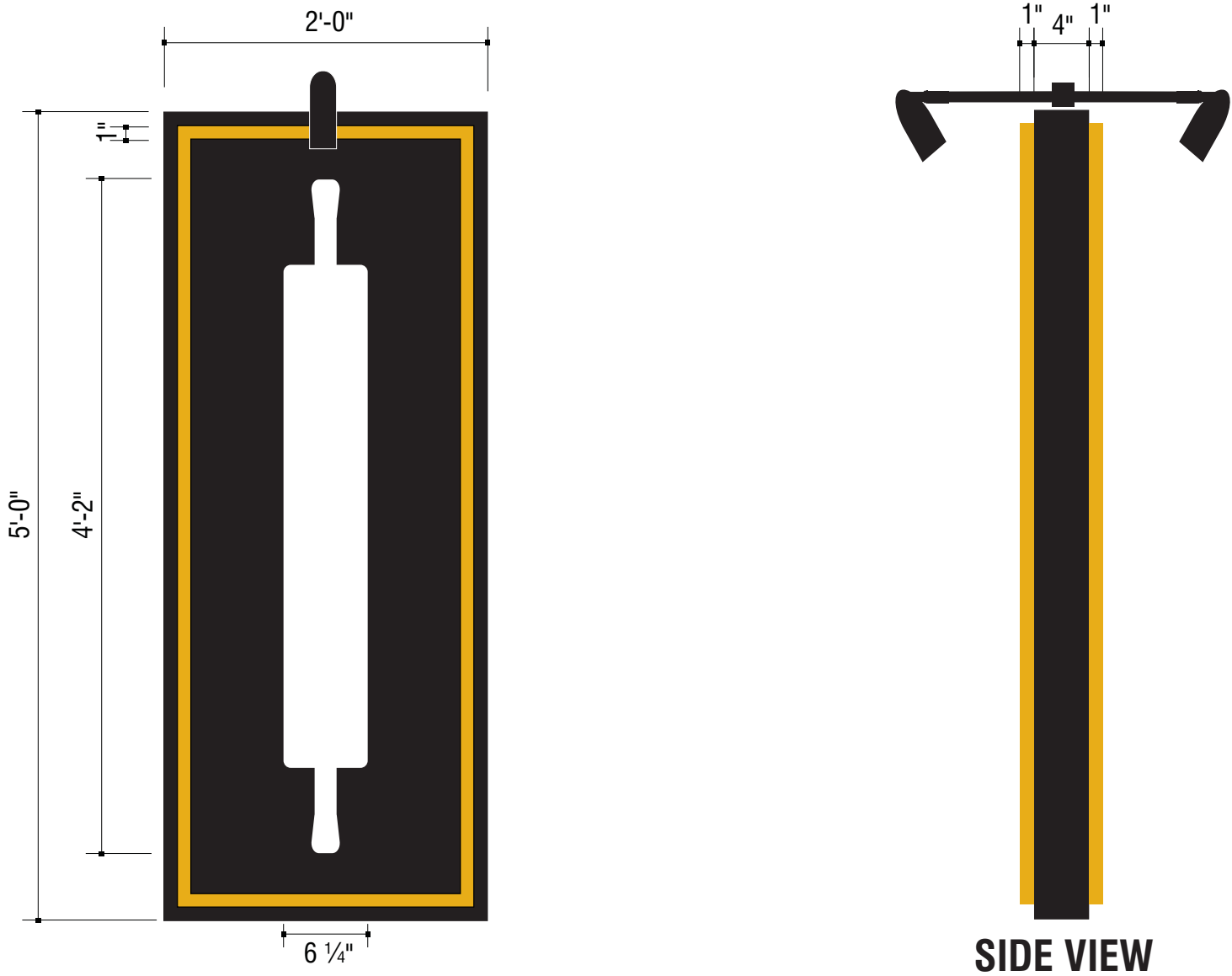
D D/F Externally Lit Blade Sign ( 1 ) Required Scale: 1"=1'-0" 10.0 Sq. Ft.
